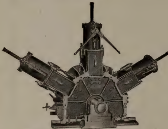
Patent Improved Wood Pulp Grinder.
